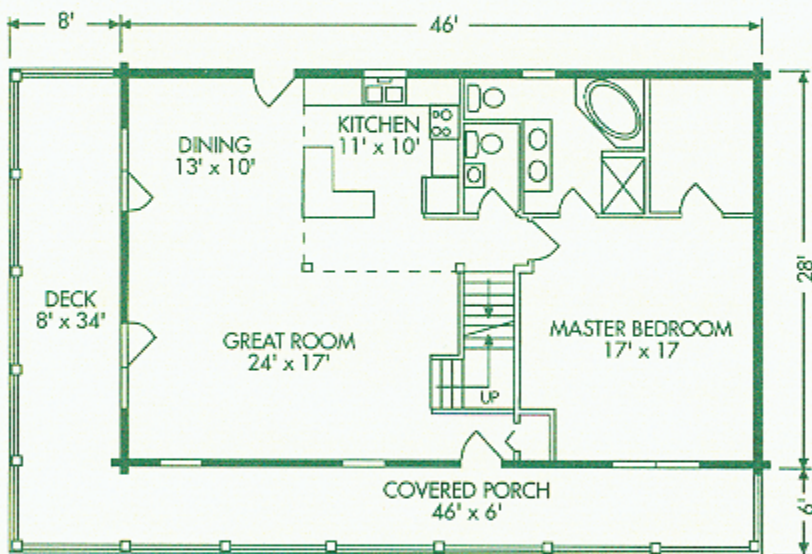
MAIN FLOOR
